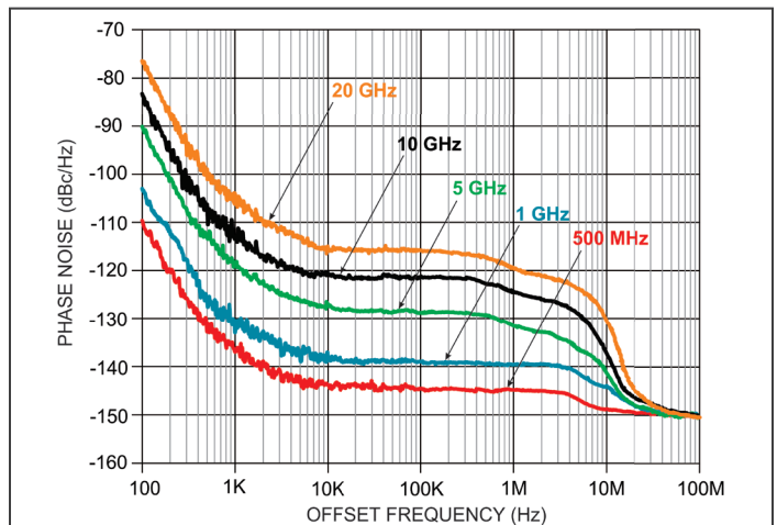
Phase Noise
