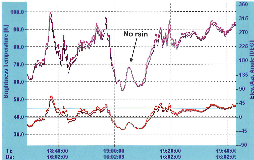
Fig. 3 Brightness Temperature
