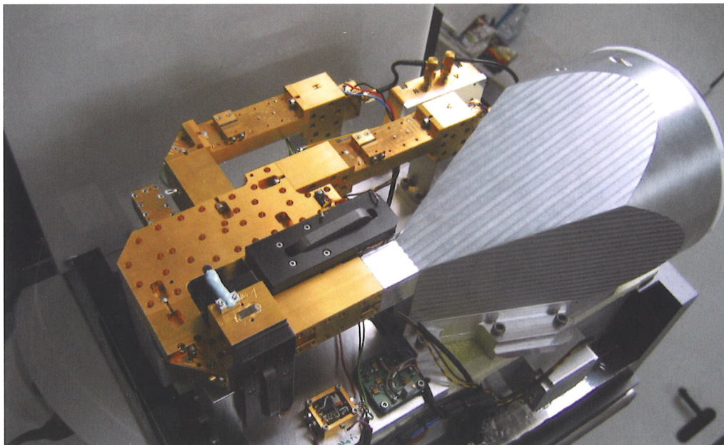
Fig. 6 RPG Double Polarization Radiometer
