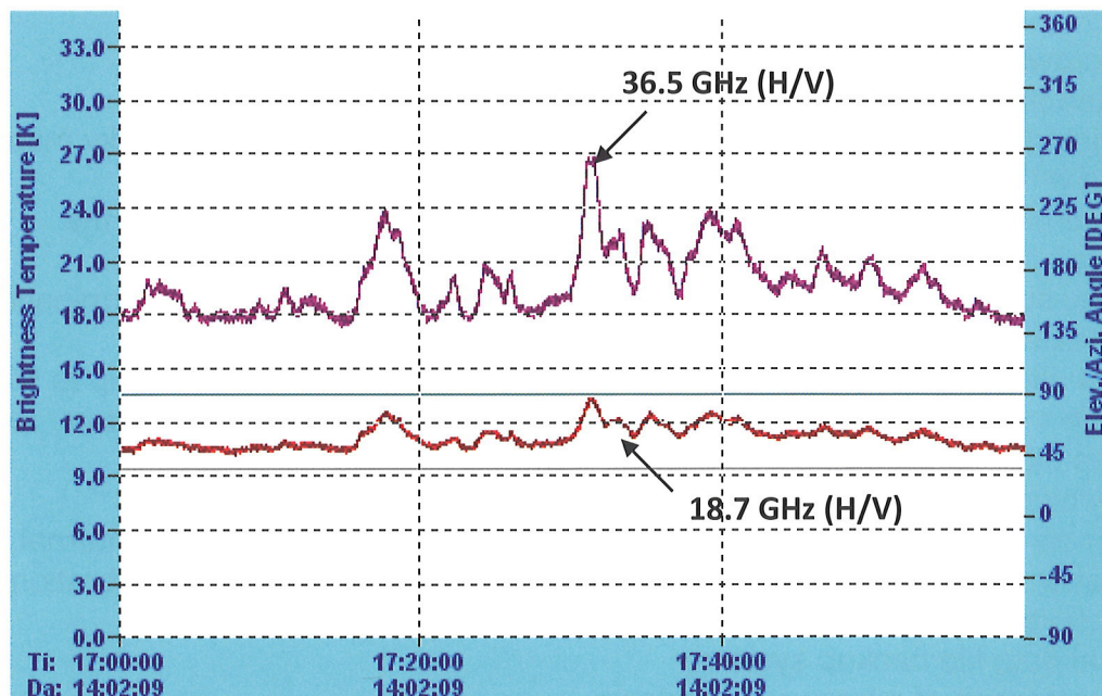
Fig. 1 Brightness Temperature time series (two frequencies, dual polarization).
