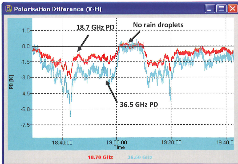
Fig. 4 Polarization Difference for rain and cloud mixtures
