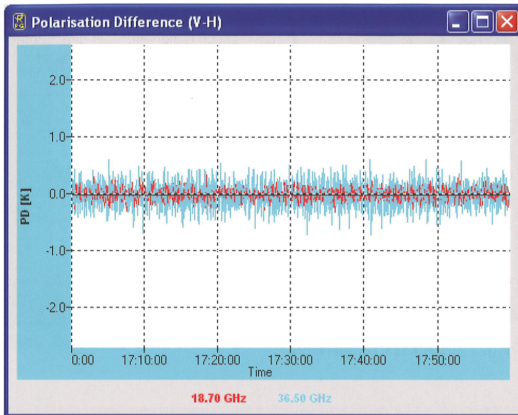
Fig. 2 Polarization difference (PD=TB v -TB h ) time series for clear sky.
