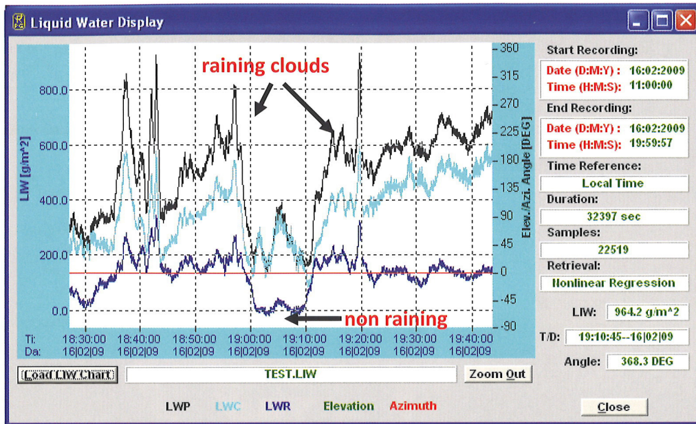
Fig. 5 Simple regression retrieval for rain and cloud fraction of LWP.
