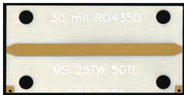
Straight microstrip test board 15c, 30 mil R04350, S/N = 51, (with actual test results).
