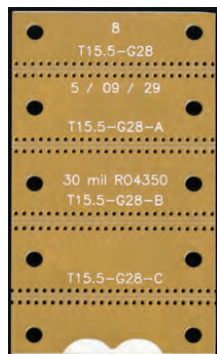
GCPWG Board
