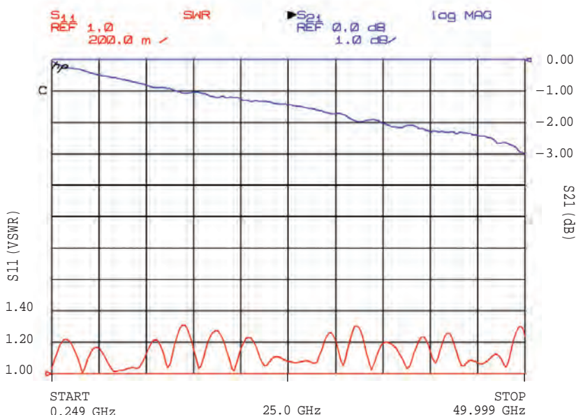
Actual test results from board 2 (Serial Number 10).
