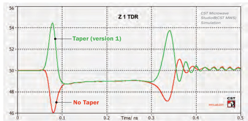
Comparison: Taper (version 1), and No Taper
